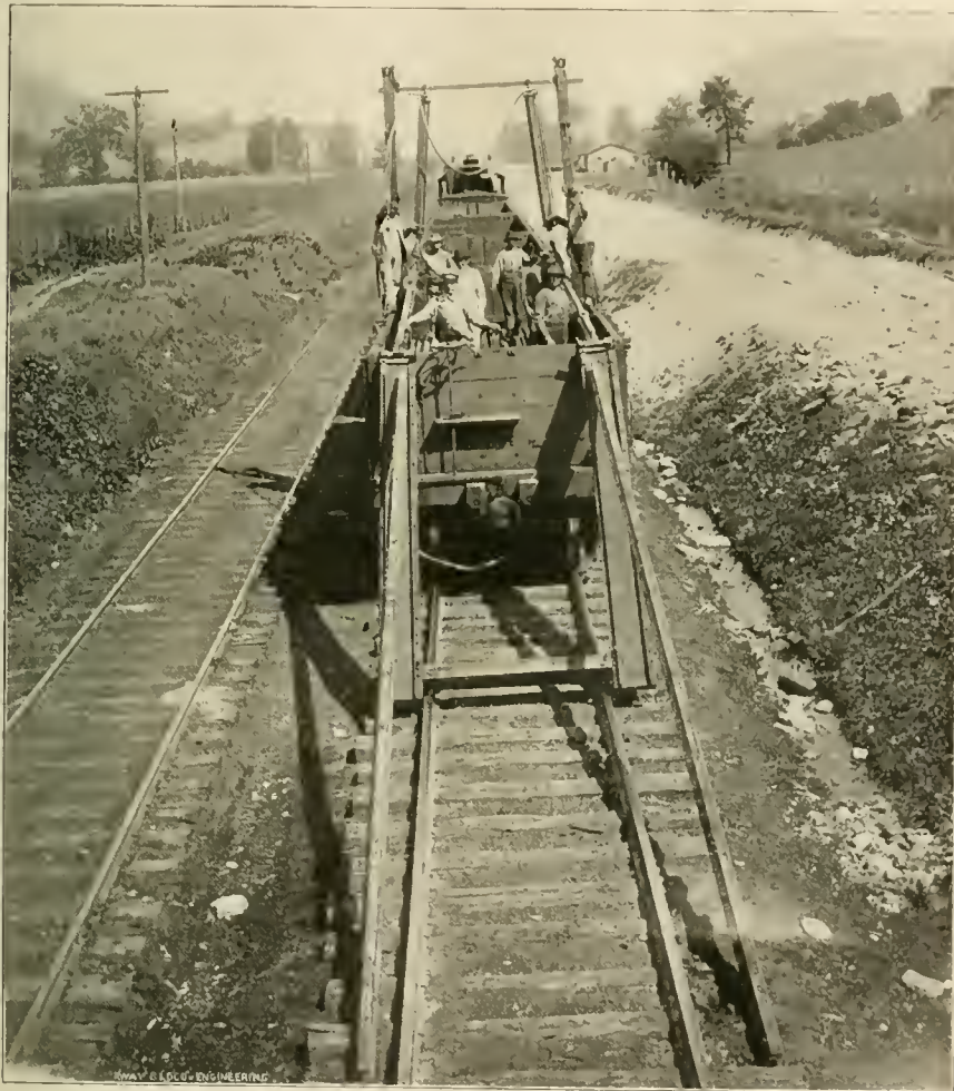
UNLOADING RAILS FROM GONDOLA WITH AIR HOISTS.
